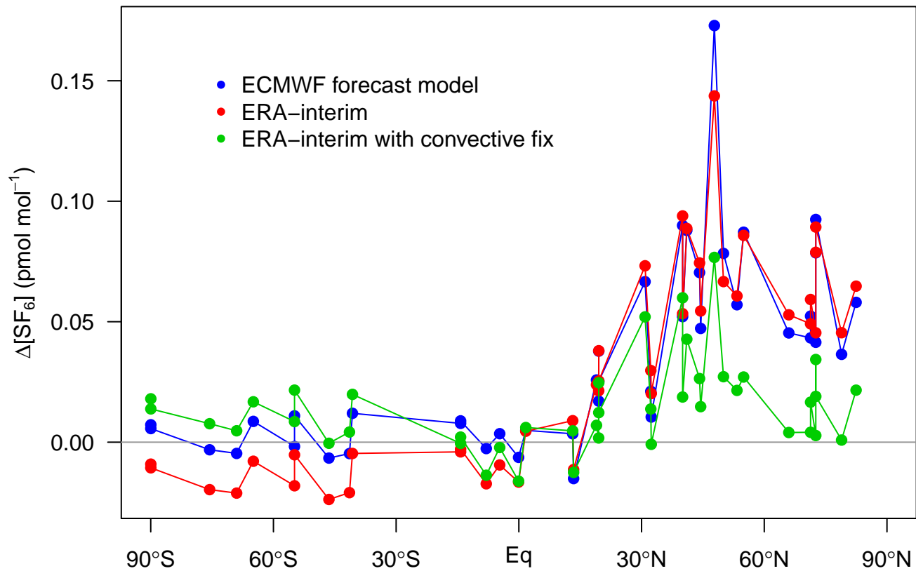
Model Minus Observed SF 6 , 2000–2008 mean by site
