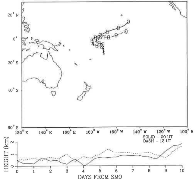
Fig. 4.10. Ten-day back isentropic trajectories arriving at SMO at 500 m on February 1, 1987, showing an example of transport from the northern hemisphere. The numbers along the trajectories give days back from SMO.
