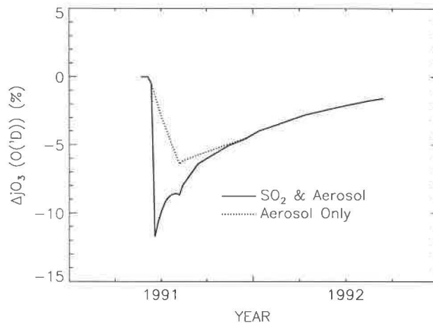
Fig. 2.13. Relative change in j_{\text{O}_3}(\text{O}(\text{}^1\text{D})) after the eruption of Mt. Pinatubo. The solid line includes the effects of direct absorption by SO 2 and scattering by sulfate aerosol; the dotted line includes aerosol only. The change is plotted relative to a 10-year climatological background.
