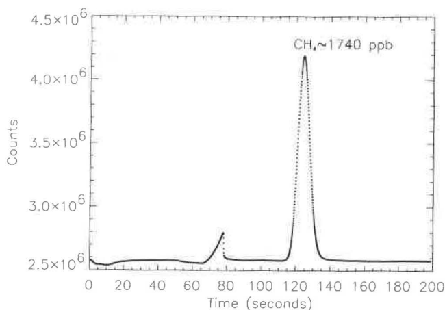
Fig. 2.10. Typical CH 4 chromatogram from MLO obtained with the new analysis system. A/D sampling rate was 10 Hz. On the y-axis, there are 10 5 counts mV -1 . Signal-to-noise is ~2000, based on a peak height of 16.8 mV and peak-to-peak noise of ~8μV. The retention time for CH 4 is 124.3 seconds, and the full-width-at-half-max is 8 seconds.
