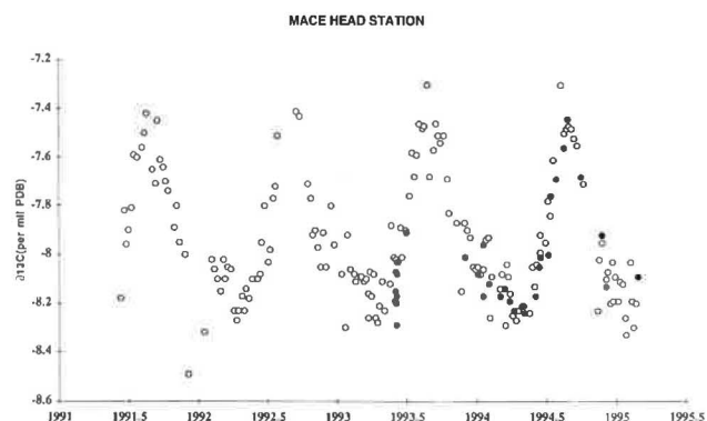
Fig. 1. Time series of \delta^{13}C of atmospheric CO_2 measured from samples of air taken at Mace Head, Ireland, by the CMDL Cooperative Flask Sampling Network (open circles) and CFR-LMCE (filled circles). The CMDL samples were analyzed by INSTAAR at the University of Colorado.
