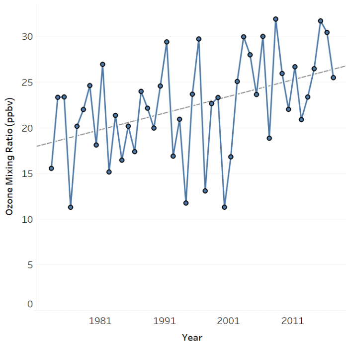
Monthly (MAY) Surface Ozone from Barrow, Alaska
