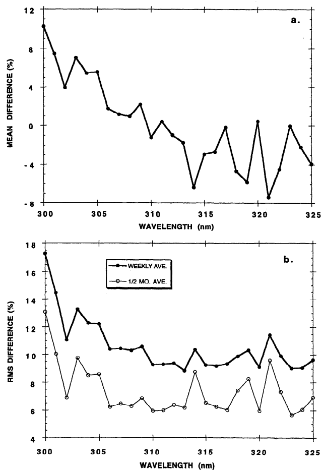
Fig. 3 a). The mean percentage difference between the weekly averaged TOMS estimated UVB irradiance and similarly averaged Brewer measured values. Positive values mean that TOMS is higher than Brewer. b). The root-mean square (rms) differences as a percentage of the mean between TOMS estimated and Brewer measured UVB irradiances for both weekly average and one-half month average time periods.
